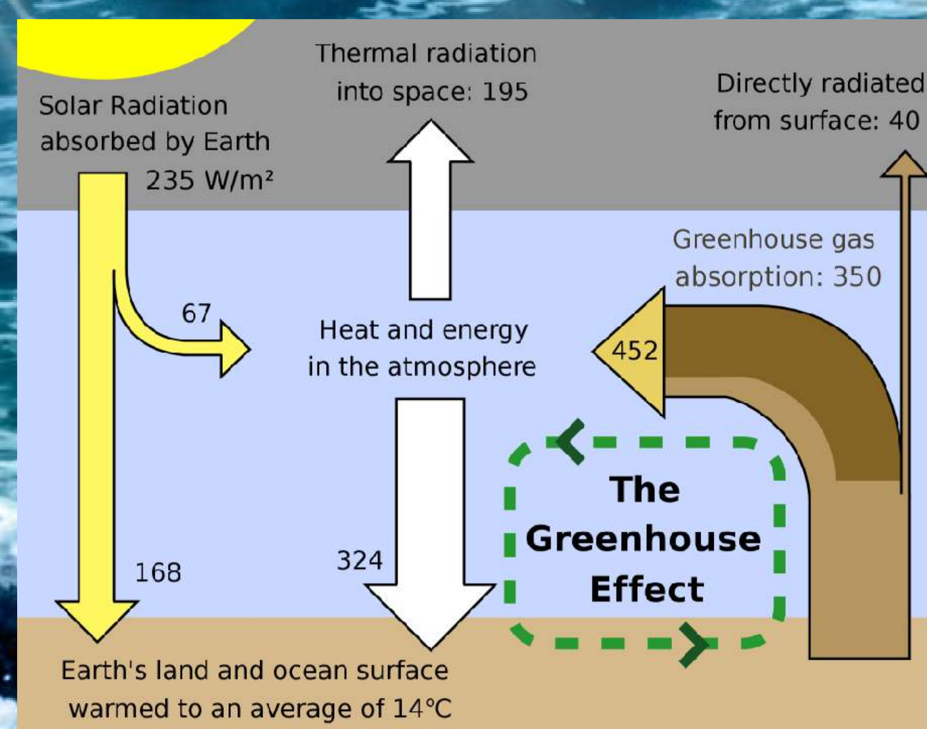
Schematic showing the energy flow between space, the atmosphere, and Earth’s surface - energy exchanges are expressed in watts per square meter (W/m 2 ). Relatively small amounts of carbon dioxide and methane generate additional atmospheric heat, which allows the air to hold more water vapour, which in turn leads to further warming. A positive feedback loop is thus created magnifying the original effect.
