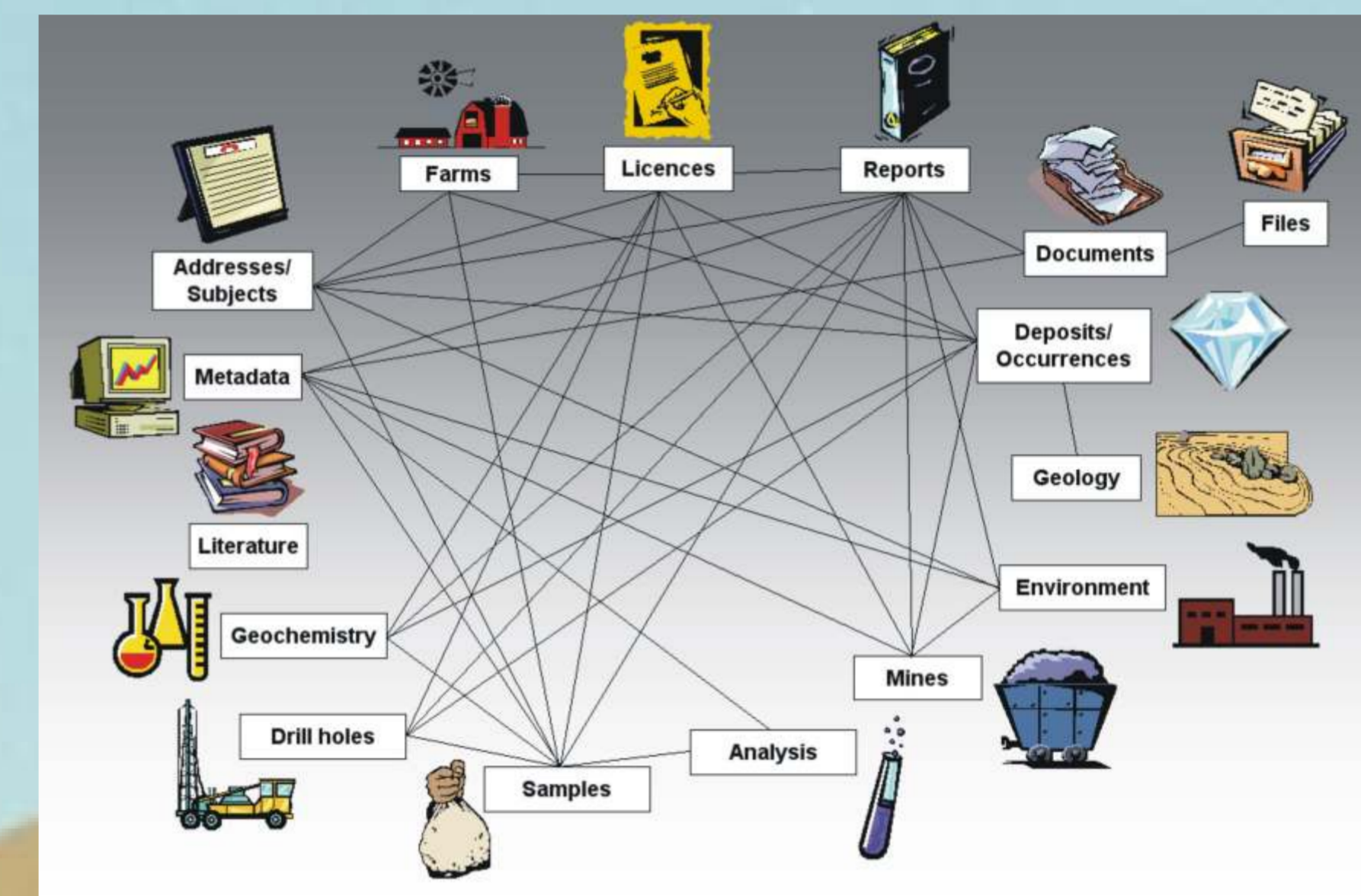
Data infrastructure of "Earth Data Namibia" - except for the literature module all the various components are interconnected in one-to-one or one-to-many relationships
