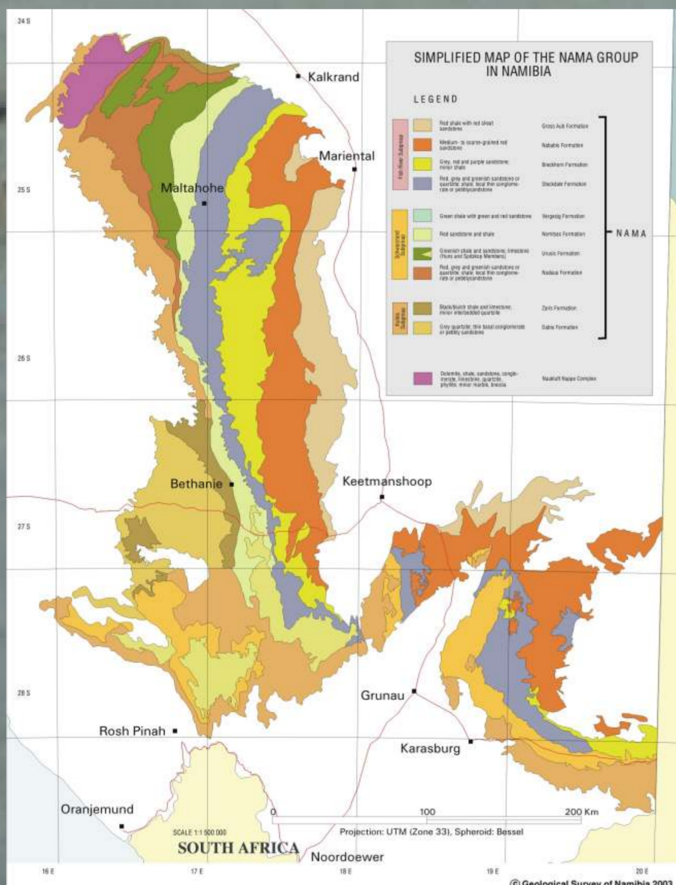
Thematic map showing the distribution of the Neoproterozoic/Cambrian Nama Group in Namibia: complementing the map is a data set, containing information in much greater detail
